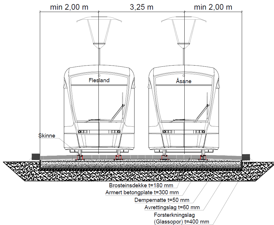
Figur 7.3-2 Normalprofil bane, fastspor
